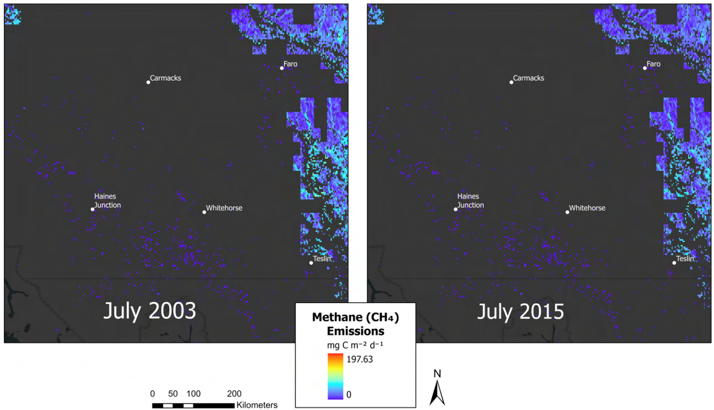
Tracking Methane Emissions Across Arctic Wetlands in Whitehorse showing July in 2003 and 2015
