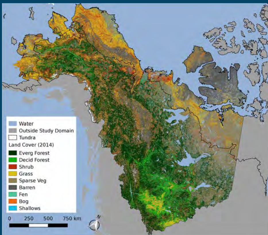
Land cover across ABoVE core domain 2014
