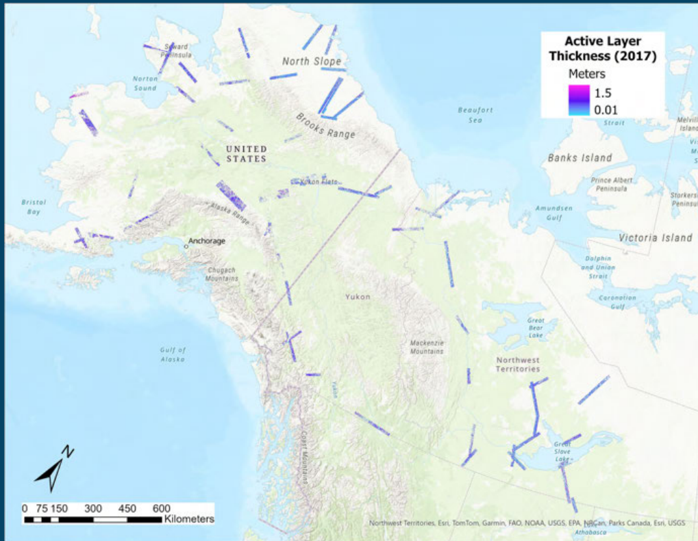
Active layer thickness measurements collected along ABoVE flight paths in 2017
