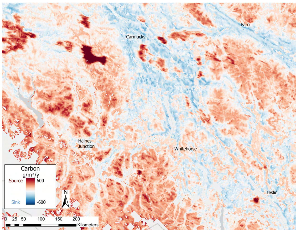
Whitehorse CO 2 Fluxes showing the Net Ecosystem Exchange and Net Ecosystem Fire from 2001-2020
