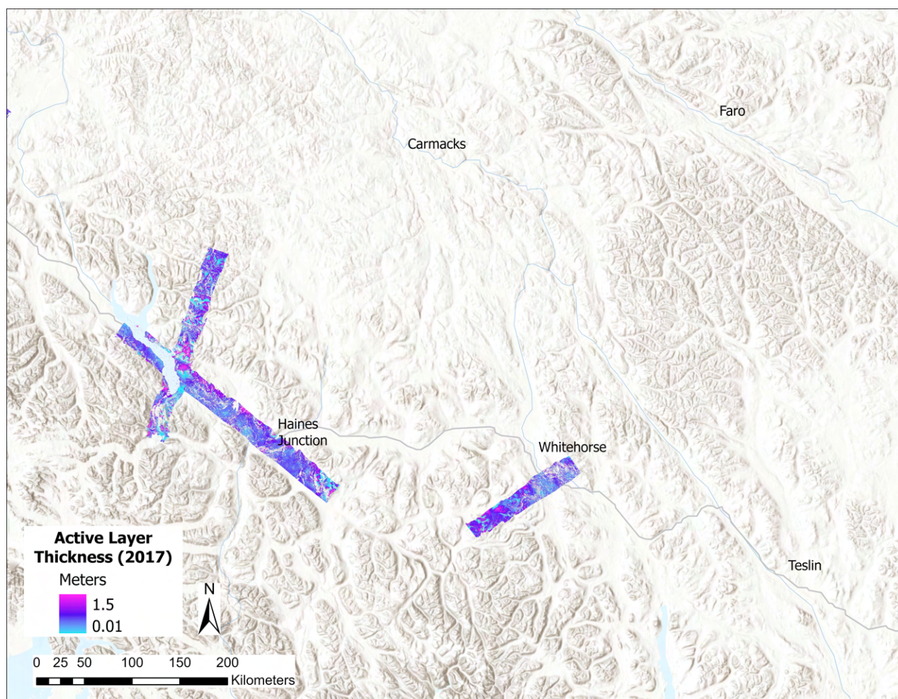
Whitehorse active layer thickness 2017
