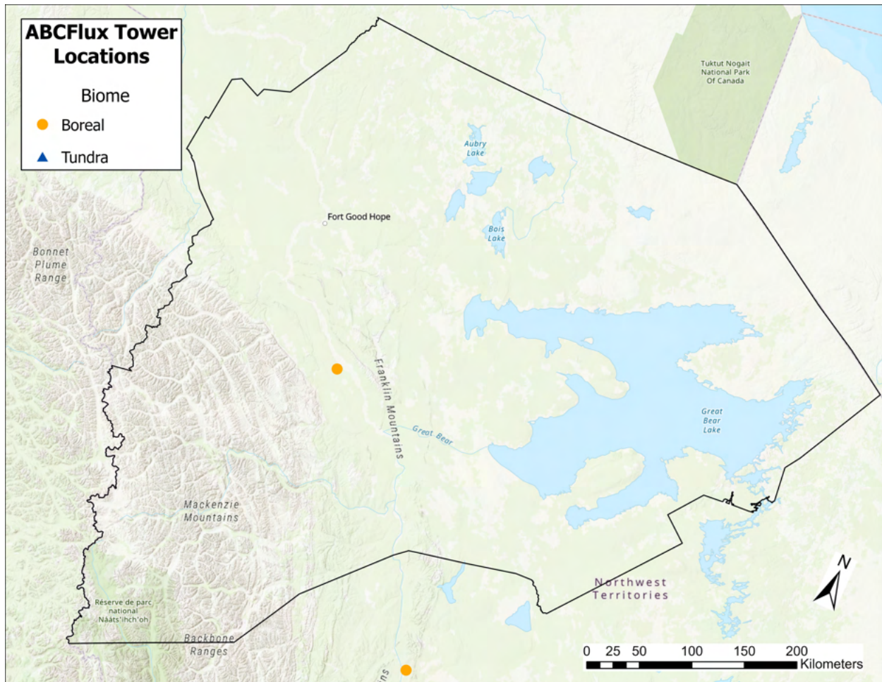
Sahtu Region ABCFlux monitoring sites, categorized by biome across tundra and boreal ecosystems
