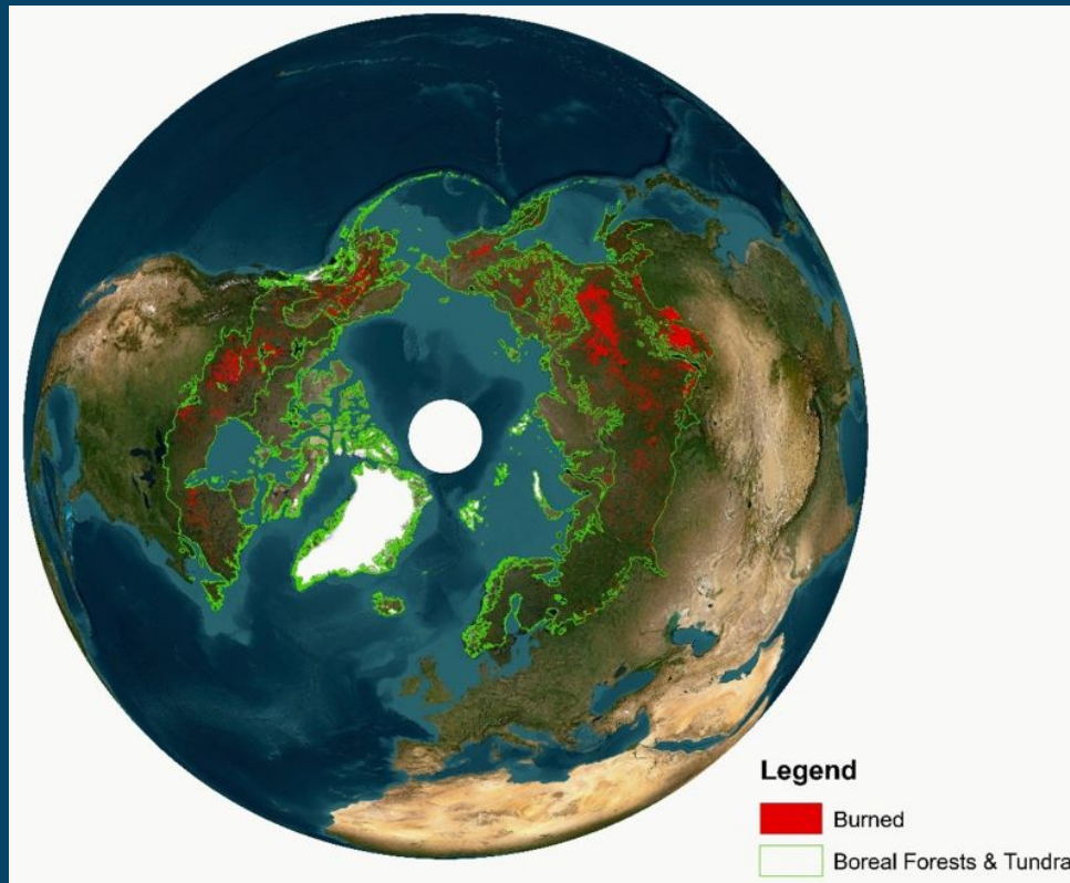
Burned area between 2002 and 2022
