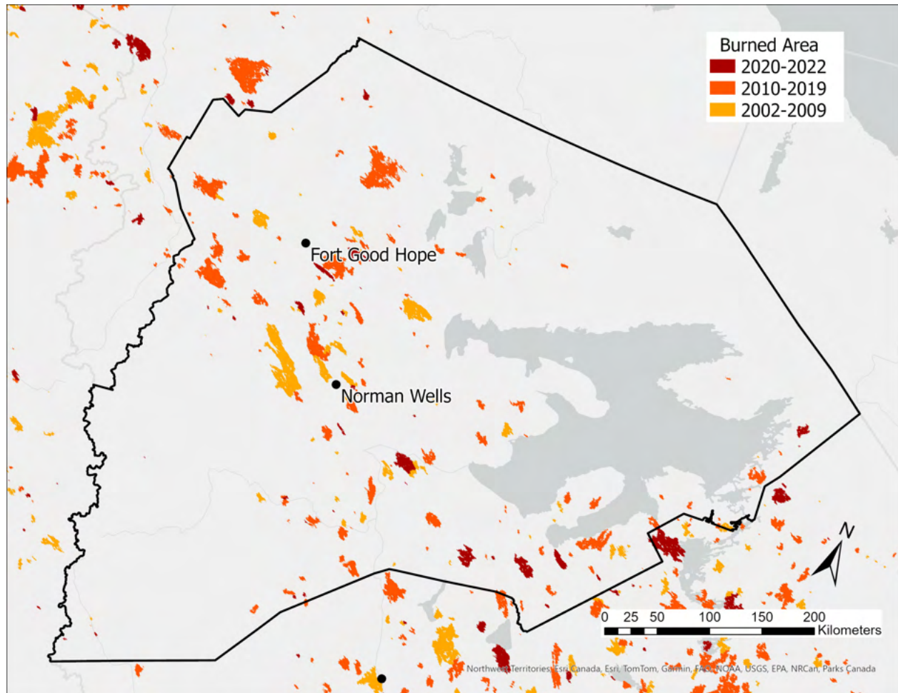
Sahtu Region burned area between 2002 and 2022
