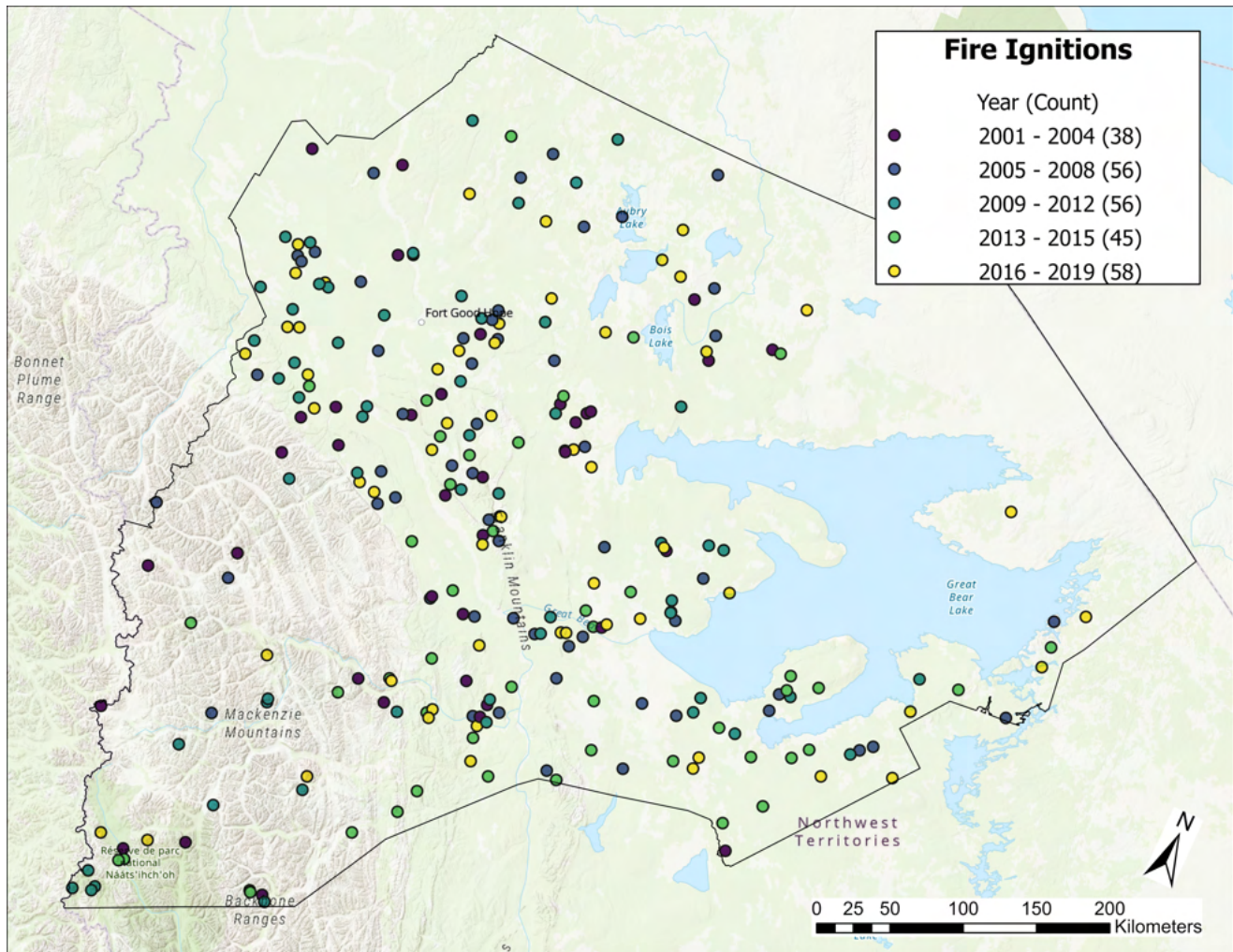
Sahtu Region Fire Ignitions, 2001 - 2019
