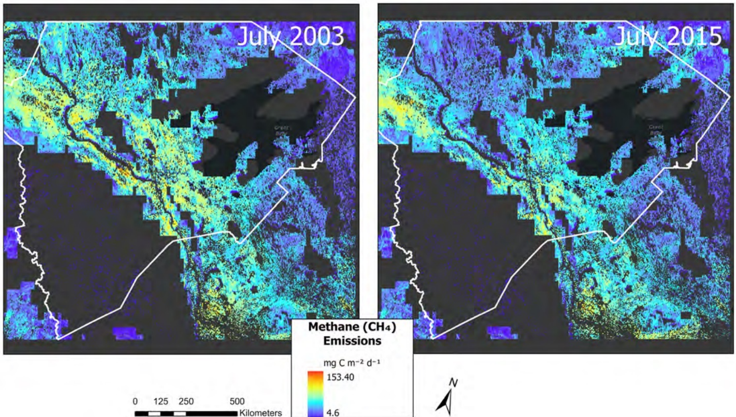
Tracking Methane Emissions Across Arctic Wetlands in the Sahtu Region showing July in 2003 and 2015
