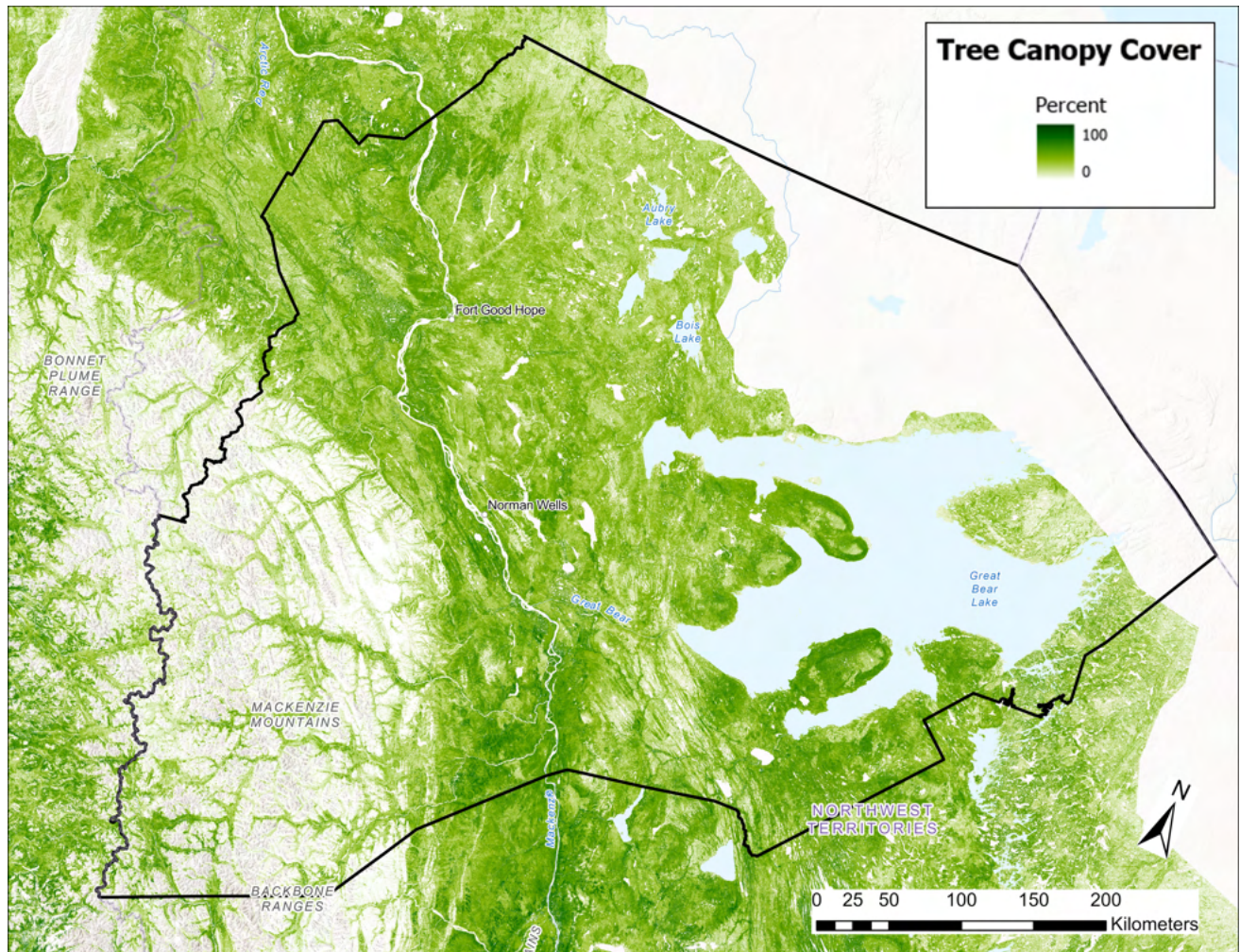
Sahtu Region Tree Canopy Cover in 2020
