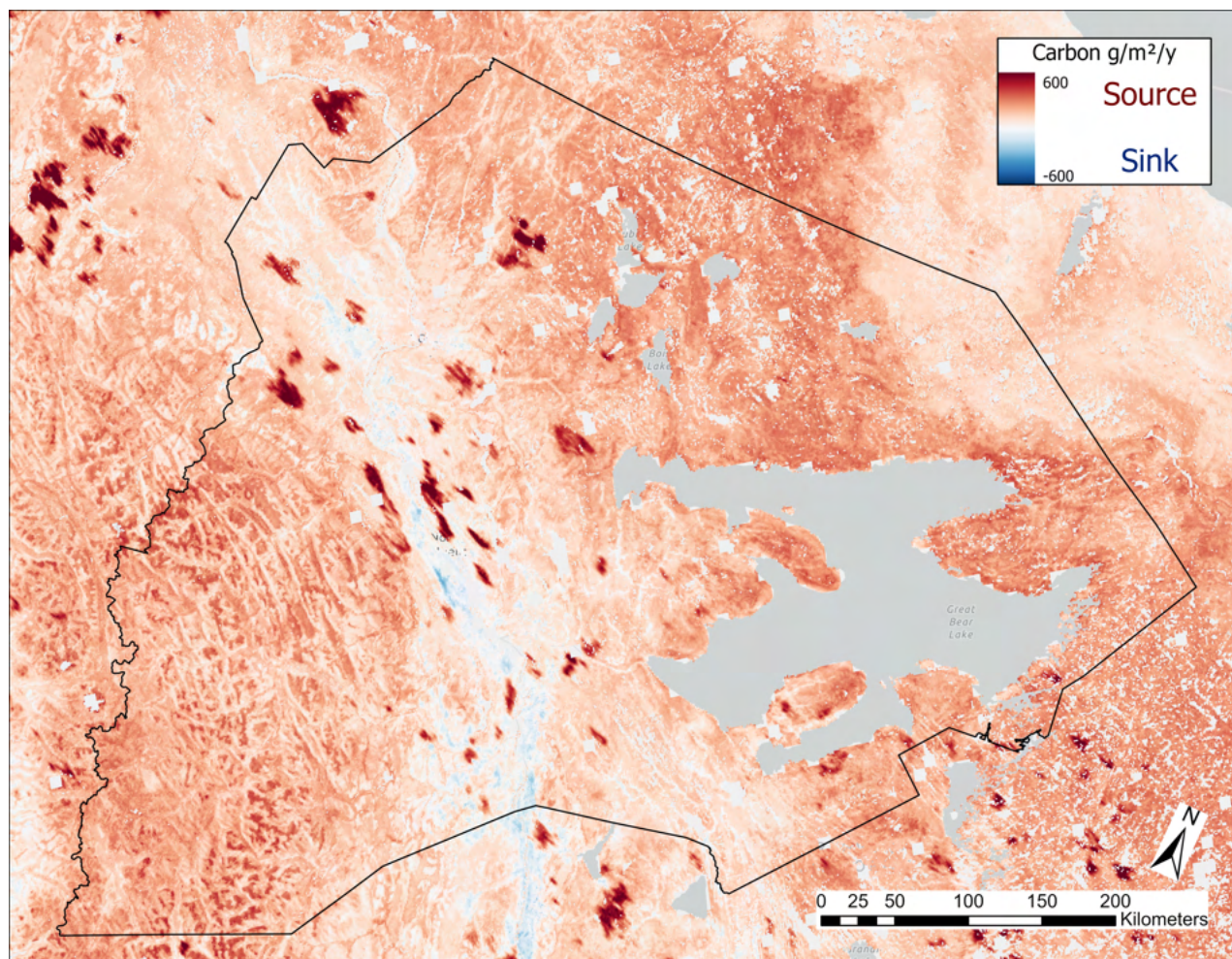
Sahtu Region CO 2 Fluxes showing the Net Ecosystem Exchange and Net Ecosystem Fire from 2001-2020
