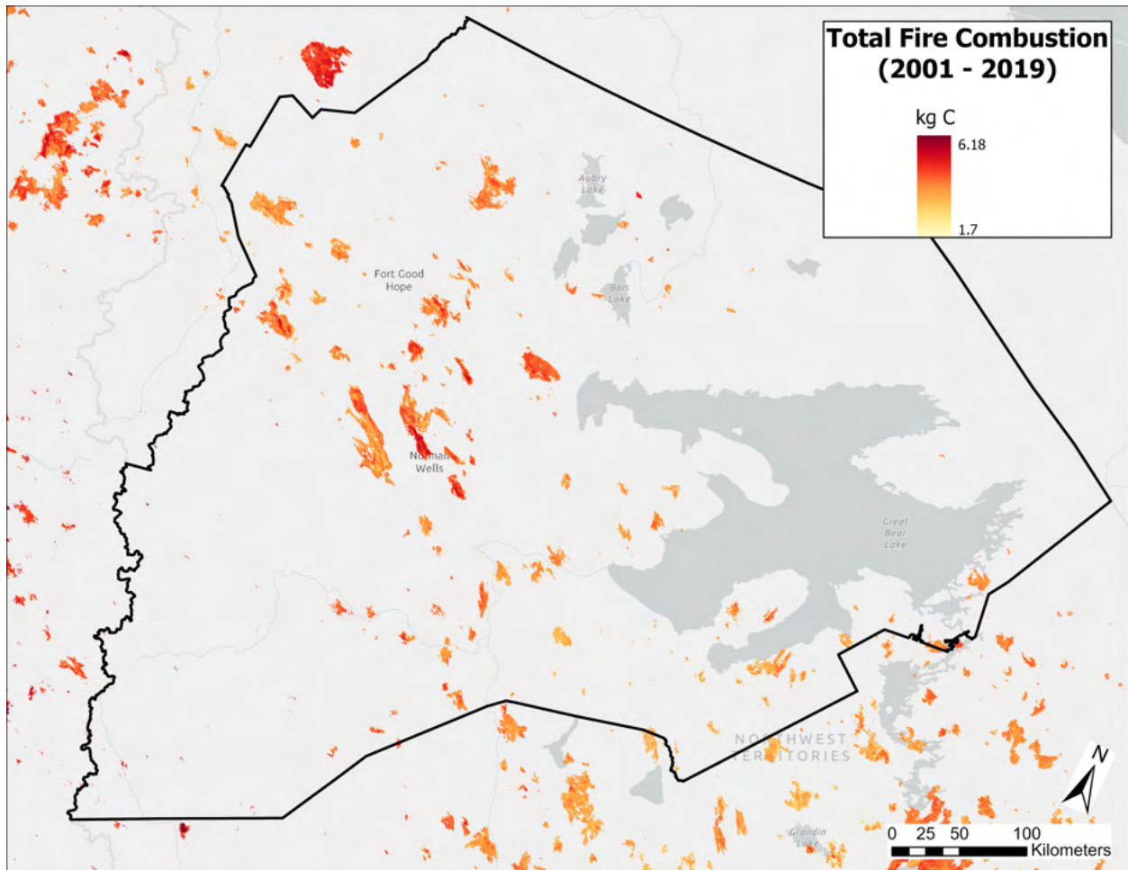
Sahtu Region total fire combustion 2001 to 2019 measured in kg C
