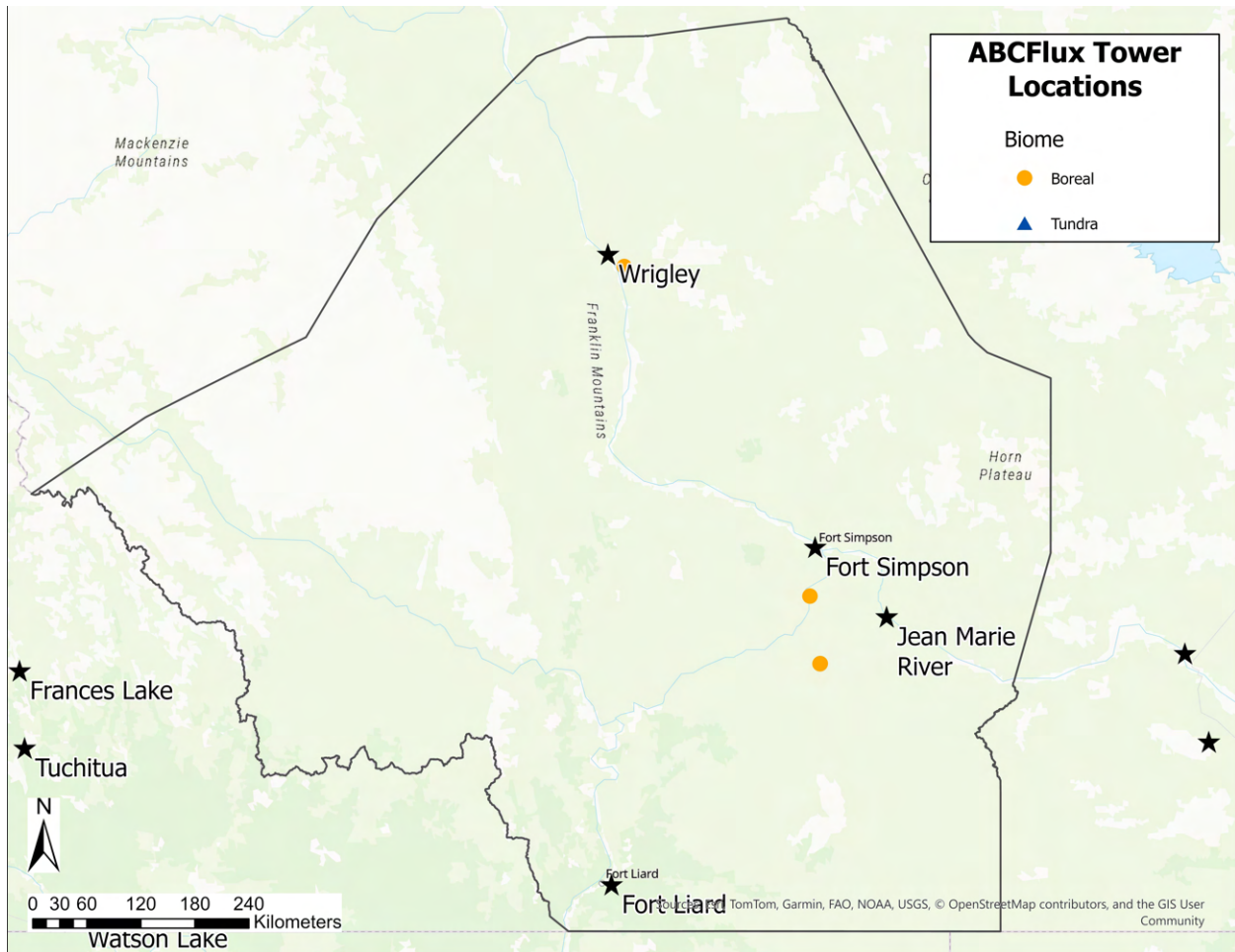
Dehcho Region ABCFlux monitoring sites, categorized by biome across tundra and boreal ecosystems
