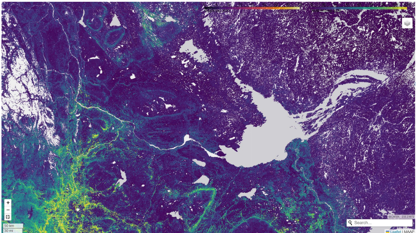
Aboveground biomass ( \text{Mg ha}^{-1} ) for boreal forest estimated from ICESat-2 imagery
