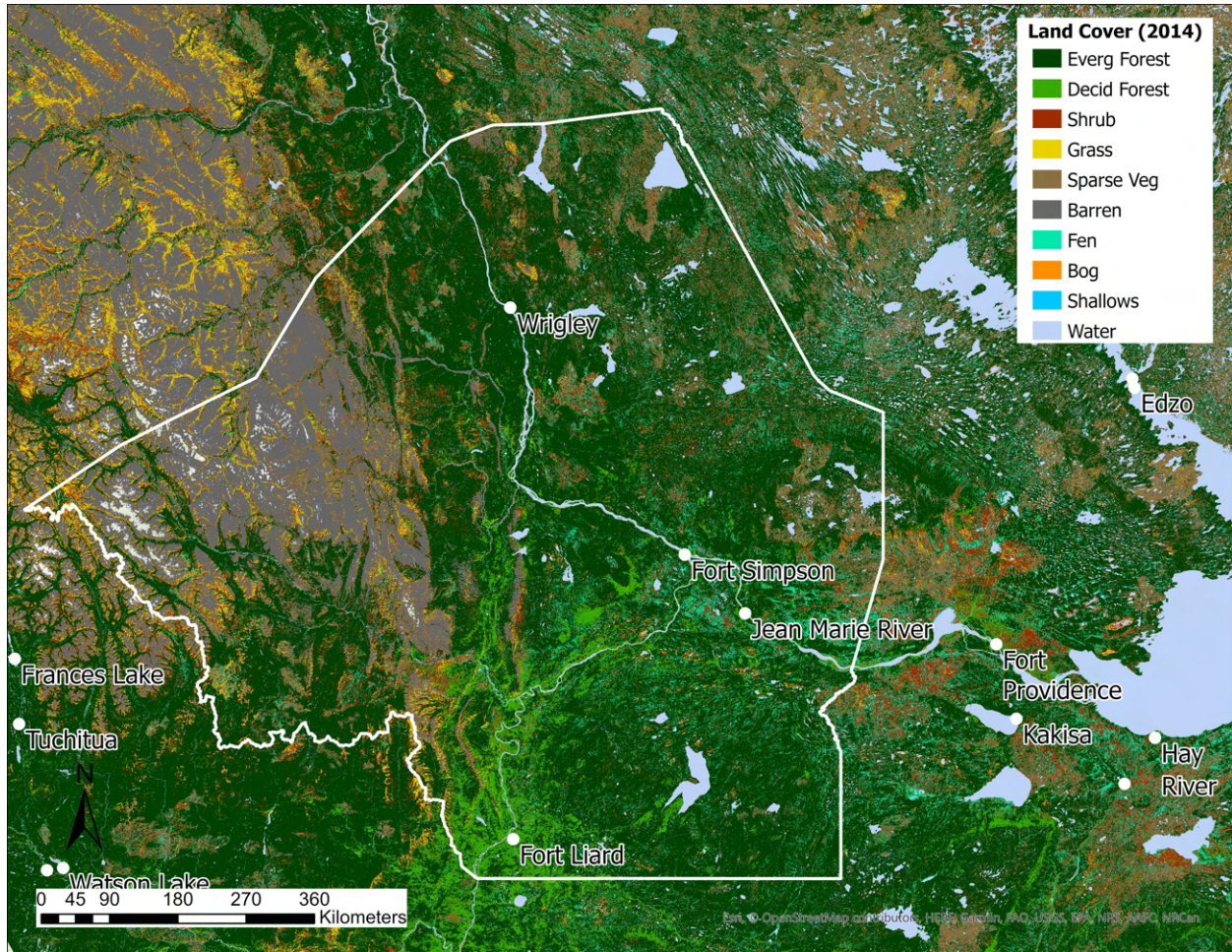
Land cover in Dehcho Region 2014
