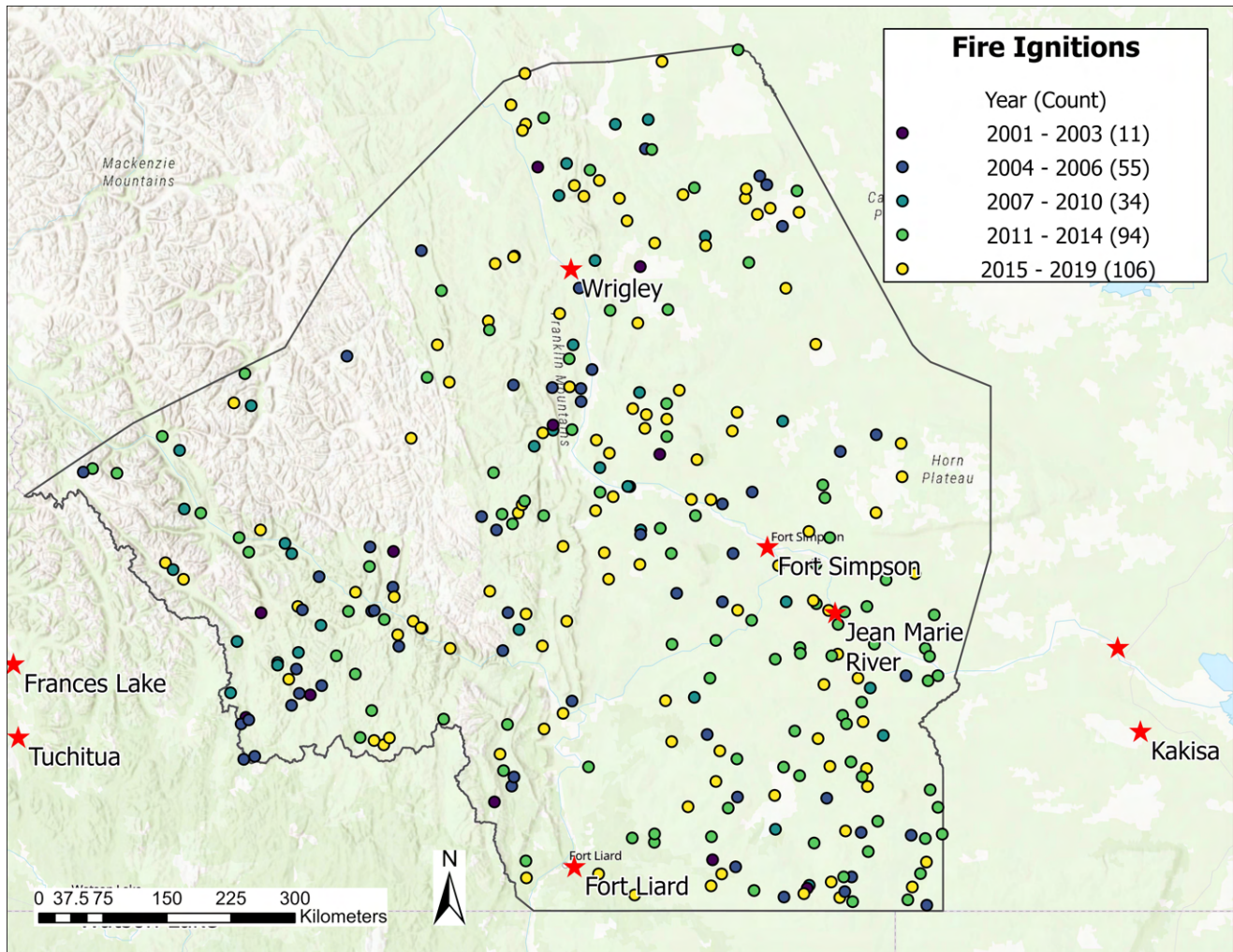
Dehcho Region Fire Ignitions, 2001 - 2019
