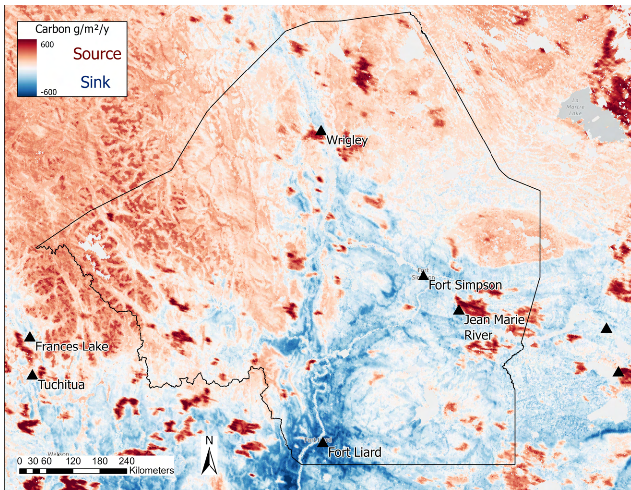
Dehcho Region CO 2 Fluxes showing the Net Ecosystem Exchange and Net Ecosystem Fire from 2001-2020
