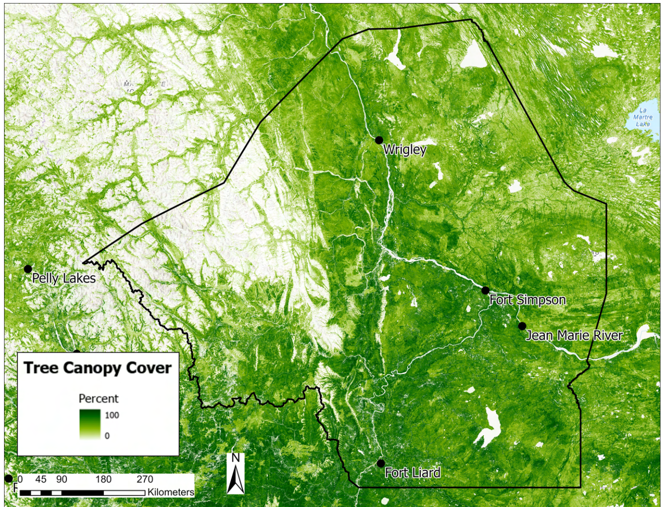
Dehcho Region Tree Canopy Cover in 2020
