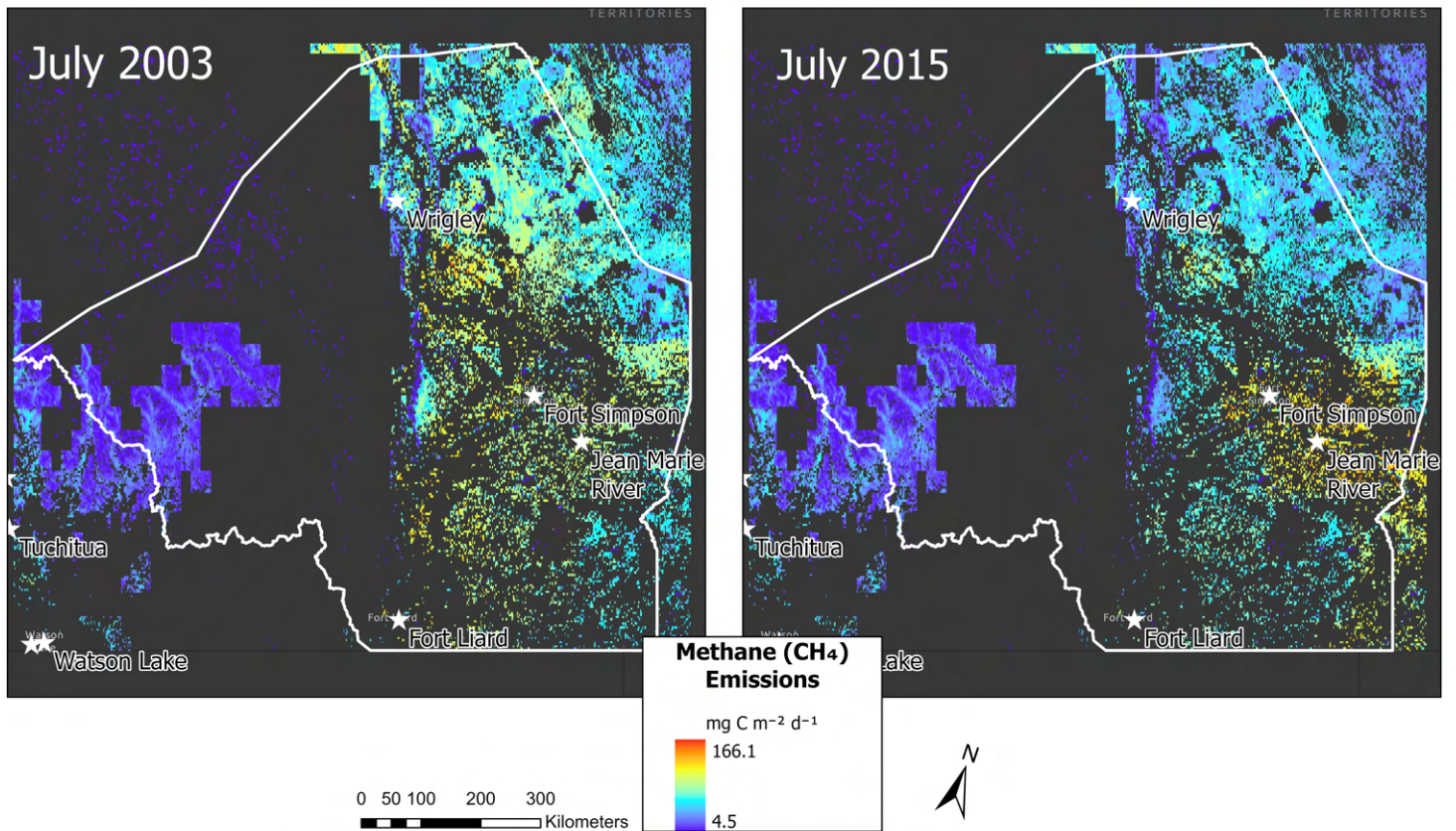
Tracking Methane Emissions Across Arctic Wetlands in the Dehcho Region showing July in 2003 and 2015
