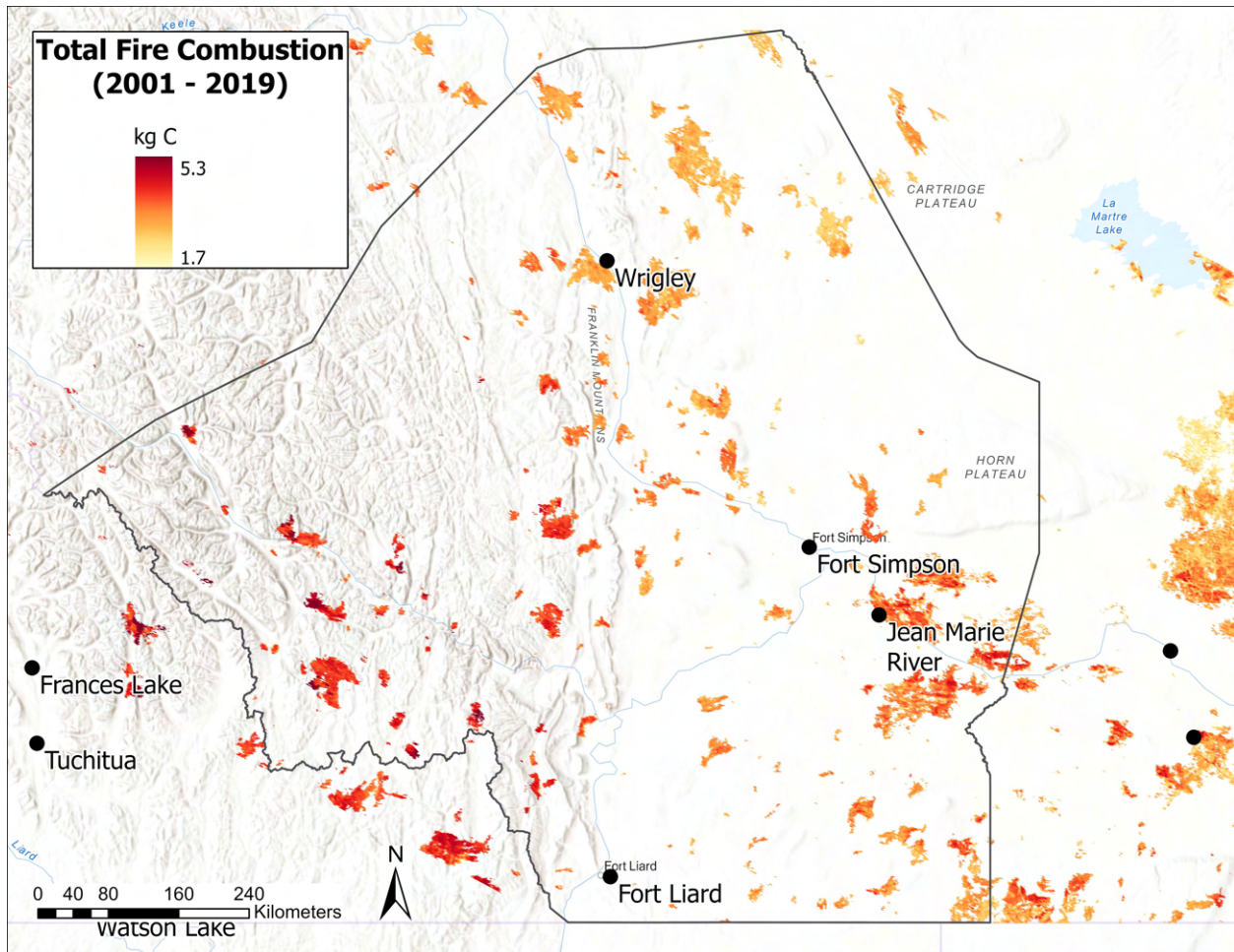
Dehcho Region total fire combustion 2001 to 2019 measured in kg C
